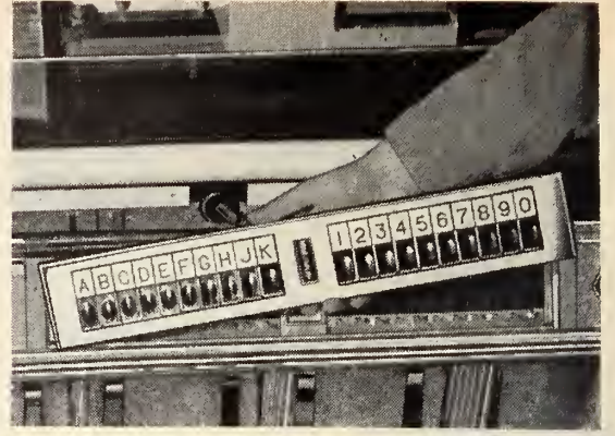
Key panel is simply removed by releasing two sliding lock fasteners.
