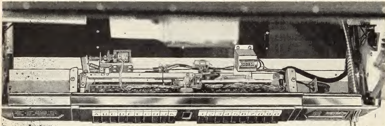
New electrical selector is designed for ease of service. Includes credit switch.
