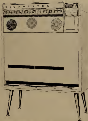
VENDO Console model CA1A (also CA2A and CA3A) 22-sel.; 850 packs all sizes; electro-mechanical push-button; 11 single cols. swing out; 11 dual-shift in rear; first-in, first-out.
