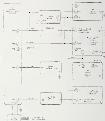
FIGURE 1 POWER DISTRIBUTION DIAGRAM
