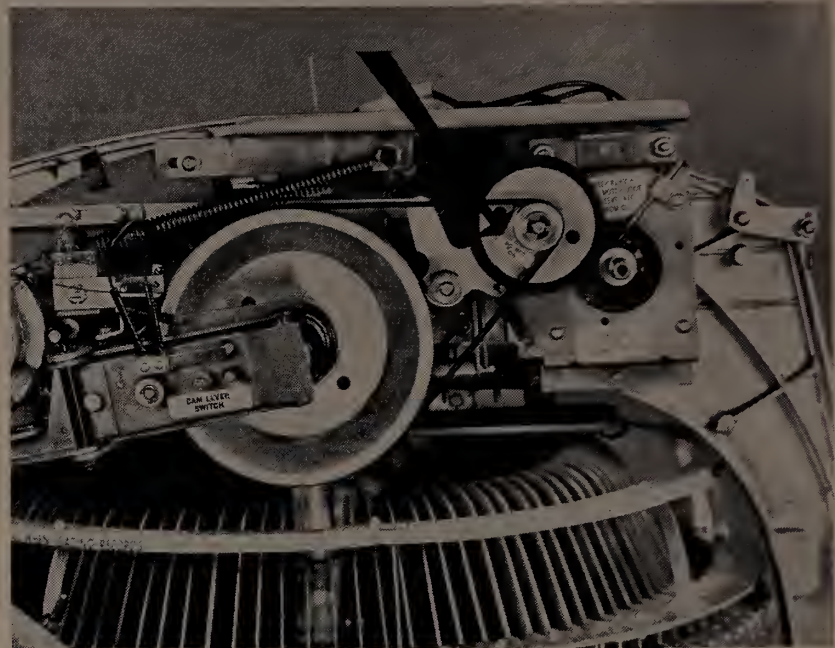
Top-rear closeup—bearing is positioned in center (hidden) of small drive wheel immediately top and right of sign reading DO NOT OIL (see black arrow).
