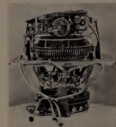
Rear view of Wurlitzer Americana's record changing mechanism.
