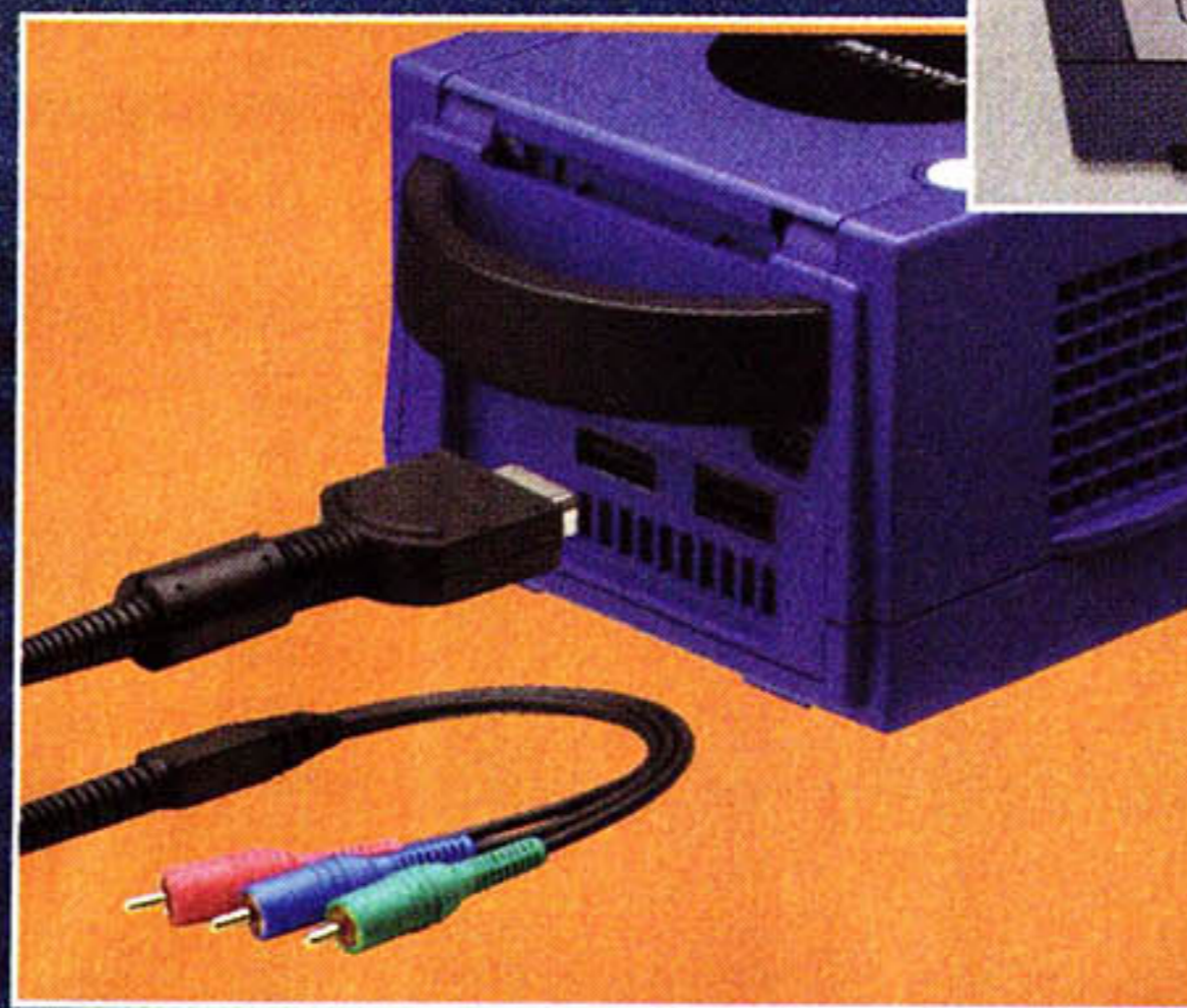
This digital A/V cable allows the GameCube to be used with high-definition televisions
