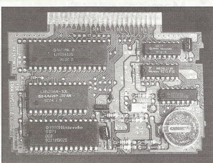
THIS IS THE BOARD IN THE MARIO KART CARTRIDGE, WITH DSP CHIP BOTTOM LEFT
