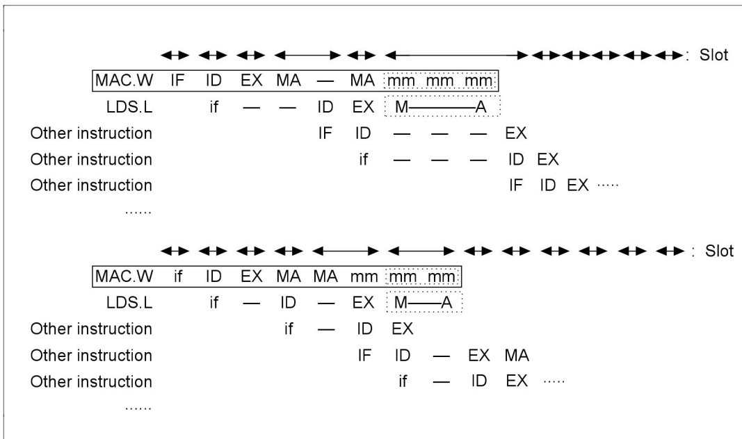
Figure 8.22 LDS.L (Memory) Instruction Immediately After a MAC.W Instruction
