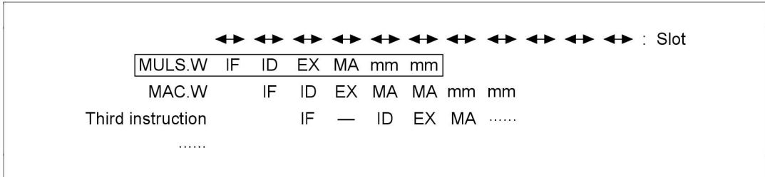
Figure 8.54 MAC.W Instruction Immediately After a MULS.W Instruction
