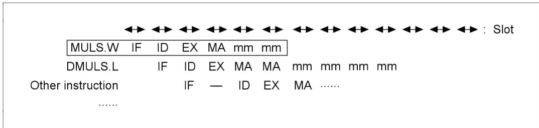
Figure 8.58 DMULS.L Instruction Immediately After a MULS.W Instruction
