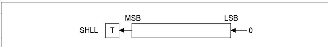
Figure 6.9 Shift Logical Left
