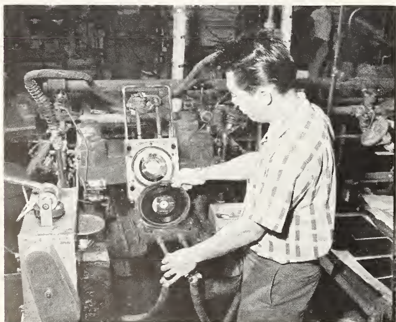
3. Employee shown operating a Compression Molding Press used in the manufacture of 45 r.p.m. phonograph records.
