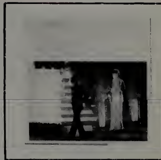
BOZ SCAGGS Down Two Then Left Columbia (7 stations)
