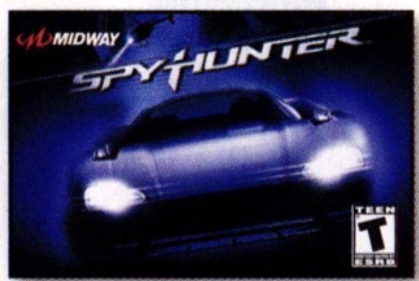
SpyHunter®
